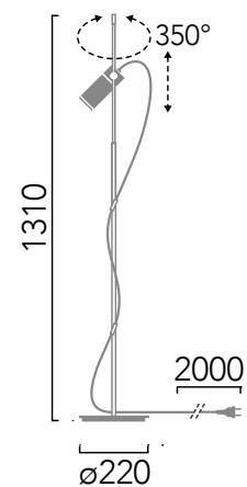
1408 - Focus Line Floor IP65
